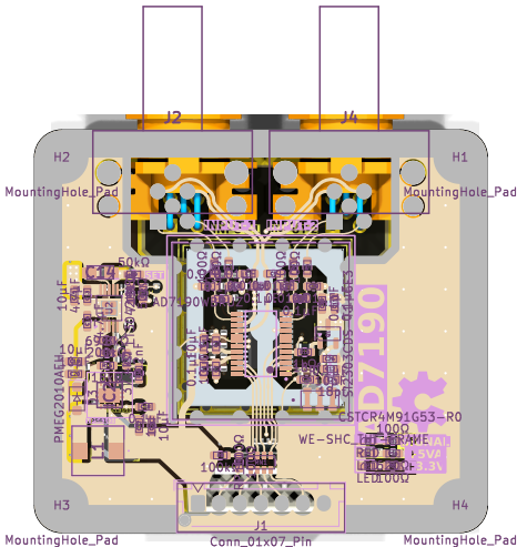
Top Assembly (Scale 1:1)
