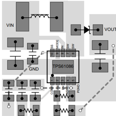
Figure 26. TPS61086 Layout Example
