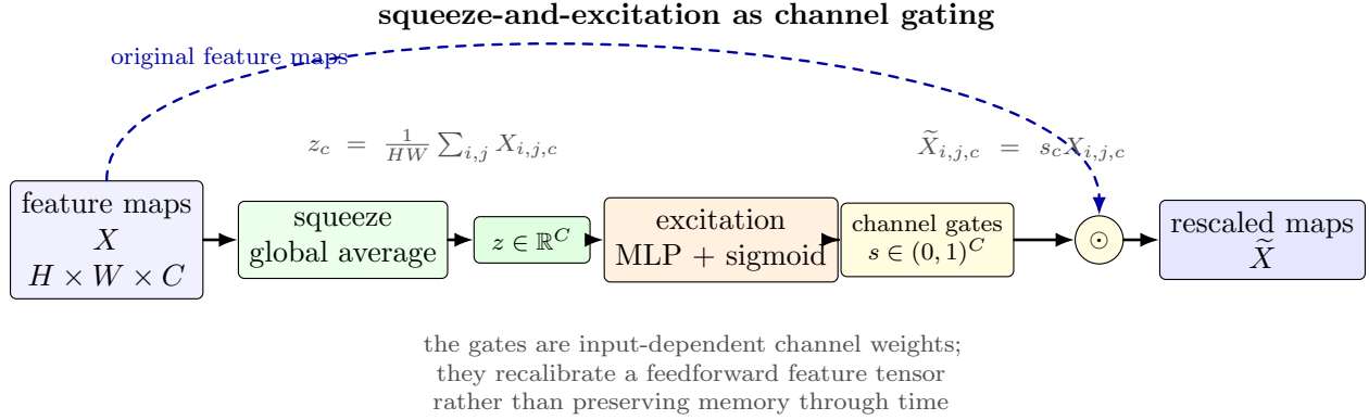
Figure 12: Squeeze-and-excitation block as a feedforward gate. The block summarizes each convolutional channel, computes sigmoid channel weights, and multiplies the original feature maps channel by channel.
