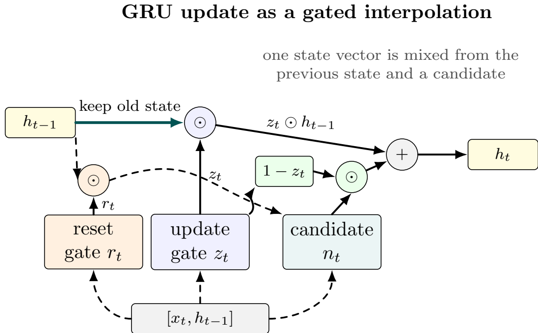
Figure 11: GRU state update schematic. The update gate controls how much previous state is retained versus replaced by a candidate, while the reset gate controls how strongly the previous state participates in forming that candidate.
