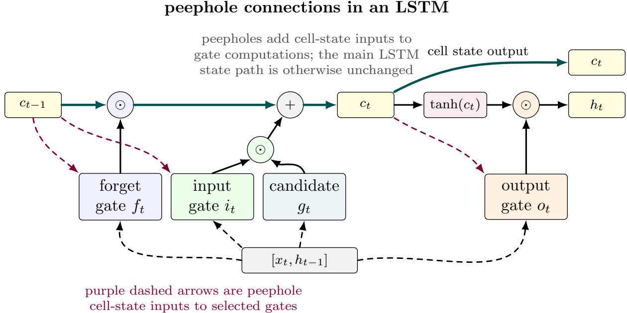
Figure 10: Peephole LSTM variant. The extra connections let gates inspect the cell state directly, for example by adding cell-state terms to forget, input, or output gate preactivations. The cell still returns both the updated cell state c_t and exposed hidden state h_t .
