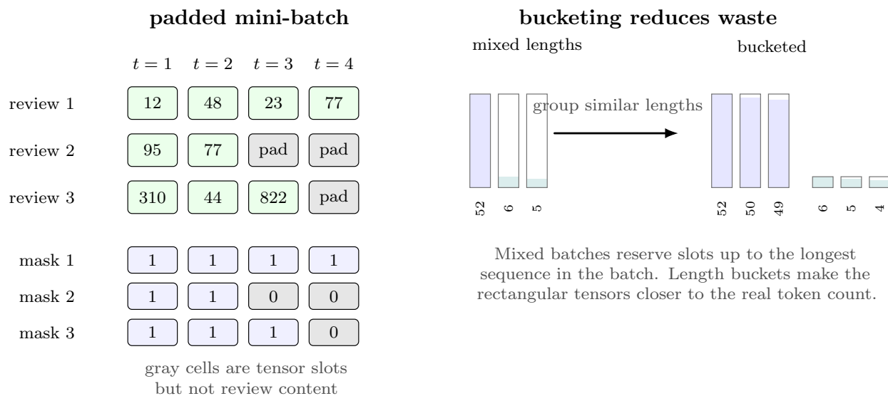
Figure 7: Padding turns variable-length reviews into rectangular tensors, and the mask identifies real token positions. Bucketing is a batching strategy: reviews of similar length are grouped so fewer tensor slots are wasted on padding.
