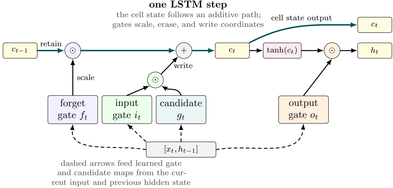
Figure 9: Simplified LSTM cell-state path. The forget gate scales the old cell state, the input gate controls a new candidate write, and the cell returns both the updated cell state c_t and exposed hidden state h_t . The output gate controls how much of the cell state becomes h_t .
