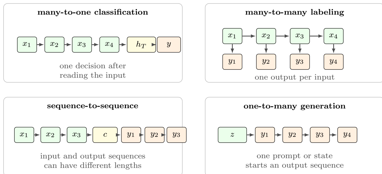
Figure 3: Common sequence task shapes. IMDB sentiment classification is many-to-one, but recurrent and attention-based sequence models also appear in aligned labeling, sequence-to-sequence prediction, and generation settings.
