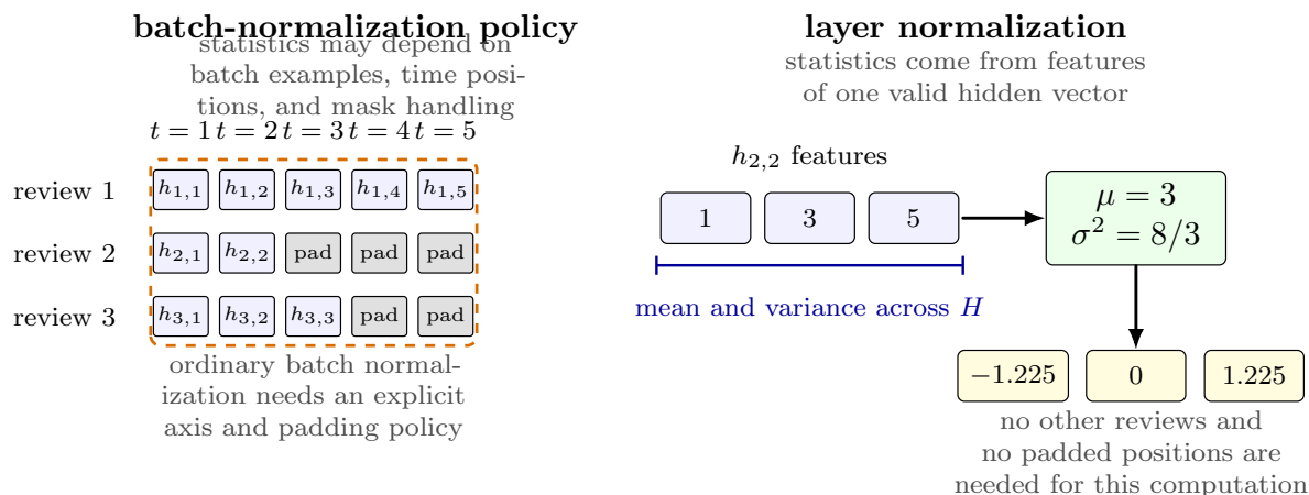
Figure 14: Normalization axes for recurrent hidden states. Batch normalization in a sequence model requires a policy for which batch and time positions supply statistics and how padded positions are excluded. Layer normalization computes statistics across the feature coordinates of one hidden vector, such as h_{2,2} = (1, 3, 5) , so it does not depend on other examples in the mini-batch.
