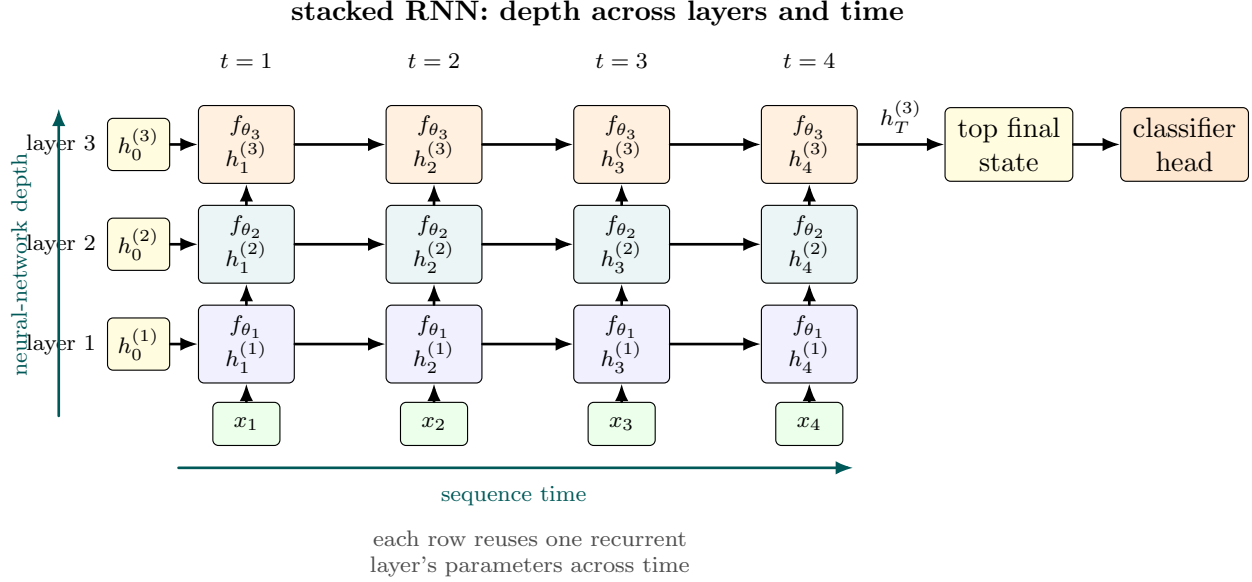
Figure 5: A stacked recurrent network unrolled through time. Horizontal connections carry each layer’s hidden state forward through the sequence, while vertical connections feed the hidden state at each time step into the next recurrent layer. The model therefore has depth across neural-network layers and length across sequence time.
