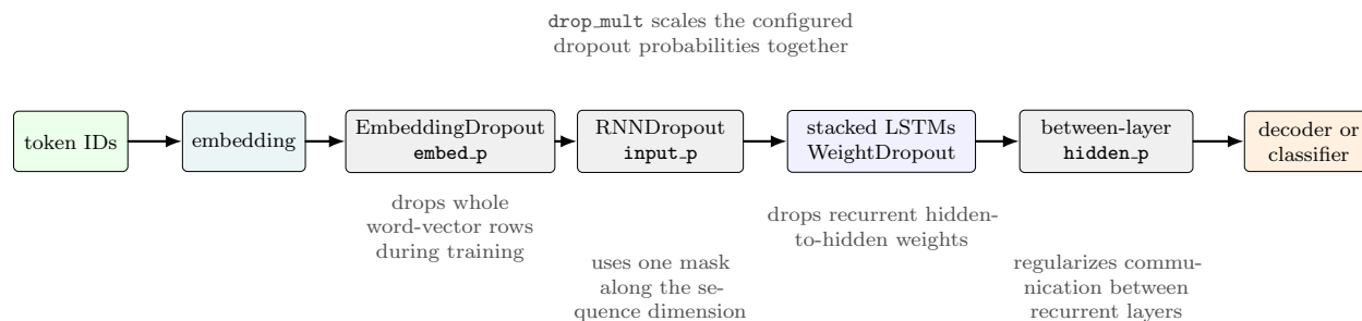
Figure 15: The fast.ai AWD-LSTM architecture combines several regularization locations instead of using one ordinary dropout layer. The public fast.ai learner examples pass AWD_LSTM as the architecture and often tune drop_mult , which scales the model’s dropout settings together.
