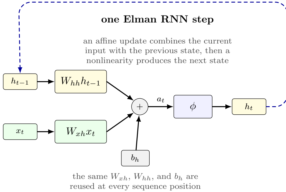
Figure 4: Simple Elman RNN cell. The current input and previous hidden state are mapped into one preactivation, a nonlinearity produces h_t , and that hidden state is passed to the next time step.
