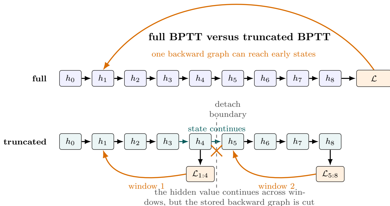
Figure 6: Backpropagation through time on an unrolled recurrent graph. Full BPTT lets a final loss send gradients through the entire stored sequence. Truncated BPTT processes shorter windows, carrying the hidden state value forward while stopping gradients at window boundaries.
