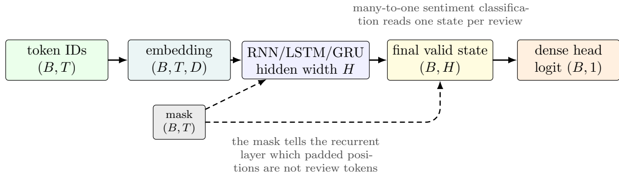
Figure 16: Tensor path for an IMDB recurrent sentiment classifier. Integer token IDs become embedding vectors, the recurrent layer reads the sequence with a padding mask, and the final valid hidden state feeds one binary sentiment logit.
