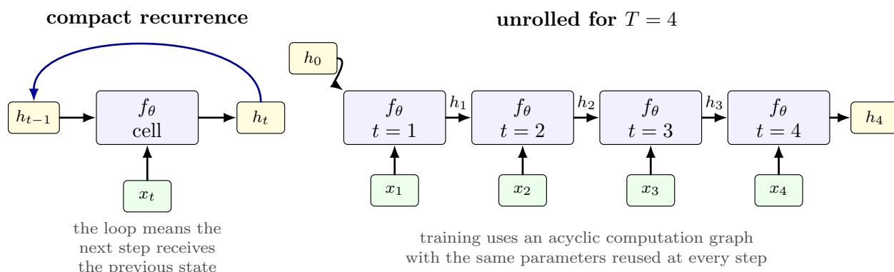
Figure 1: Compact and unrolled views of the same recurrent computation. The compact loop is notation for repeatedly applying the same state-update function; for a fixed sequence length, the training graph is unrolled through time.
