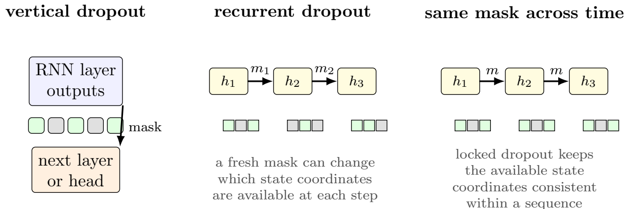
Figure 13: Dropout locations and mask-sharing choices for recurrent models. Vertical dropout masks connections between layers or before a classifier head; recurrent dropout masks the state pathway; same-mask recurrent dropout reuses one mask across time for a given sequence.
