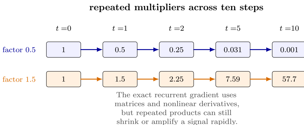
Figure 8: Toy repeated-gradient multipliers. A factor below one quickly erases a backward signal, while a factor above one can make it unstable. This figure illustrates the arithmetic behind vanishing and exploding gradients.
