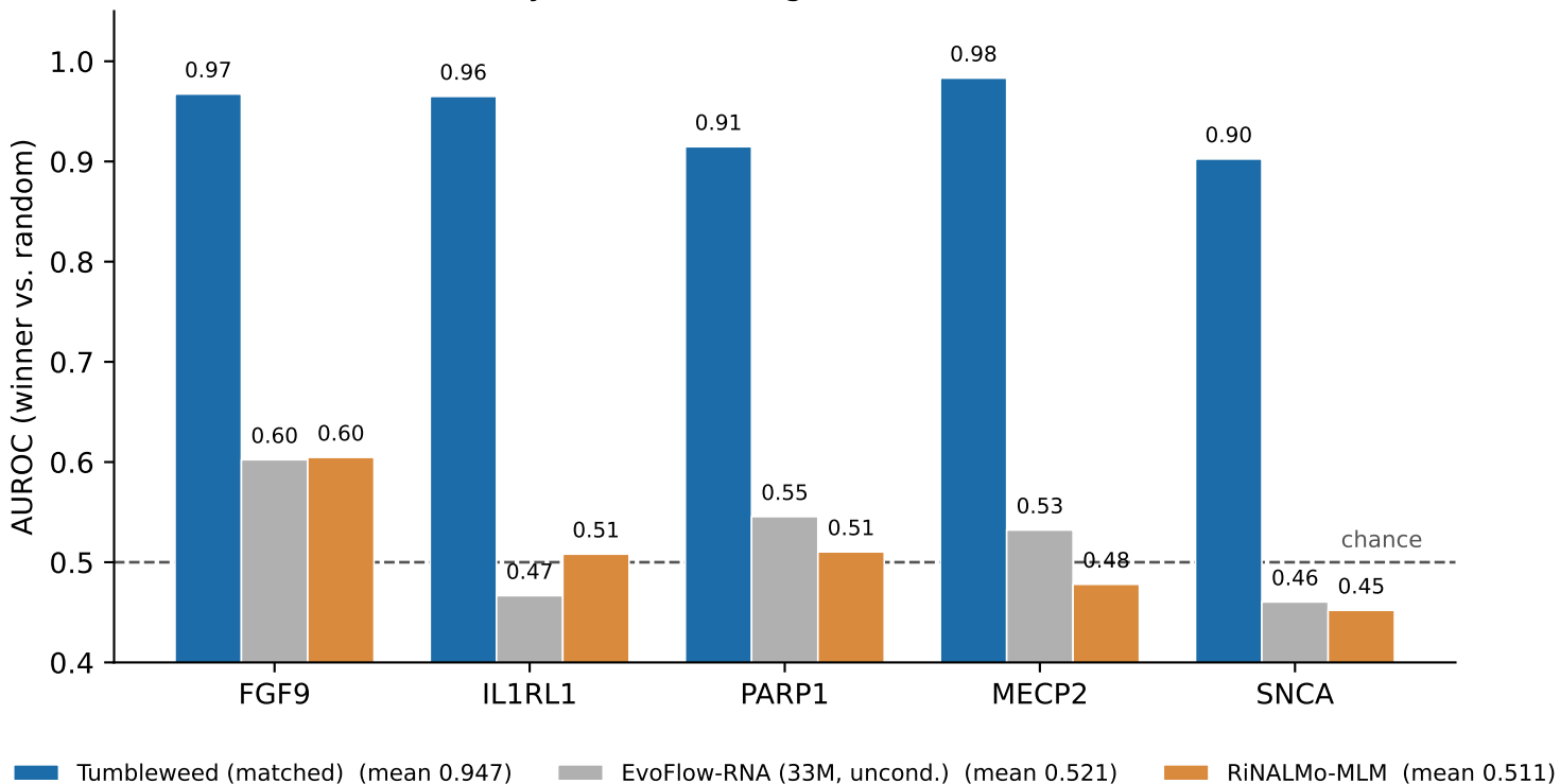
Tumbleweed-RecoveryBench: ranking true SELEX winners above random
