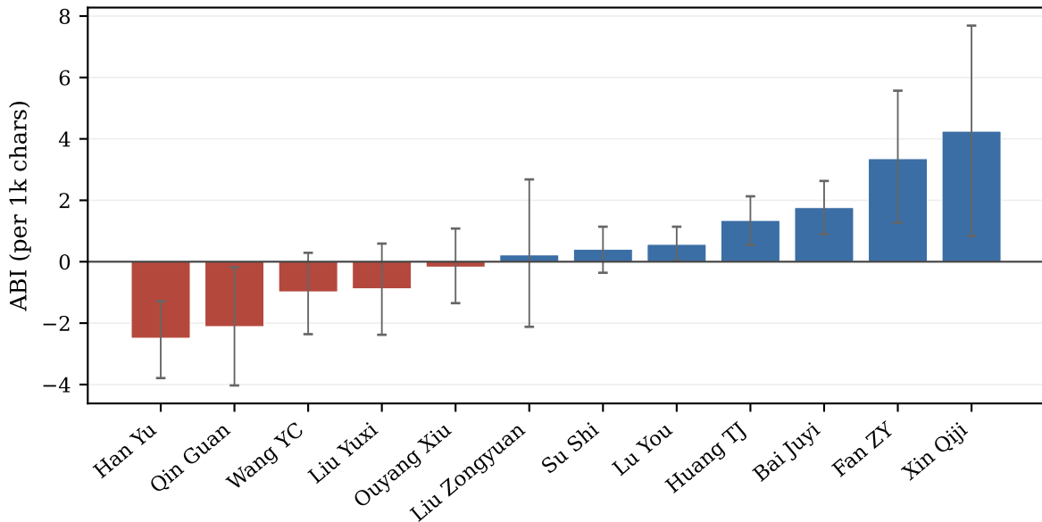
Author-level ABI with 95% bootstrap CI (n=12 cohort officials)
