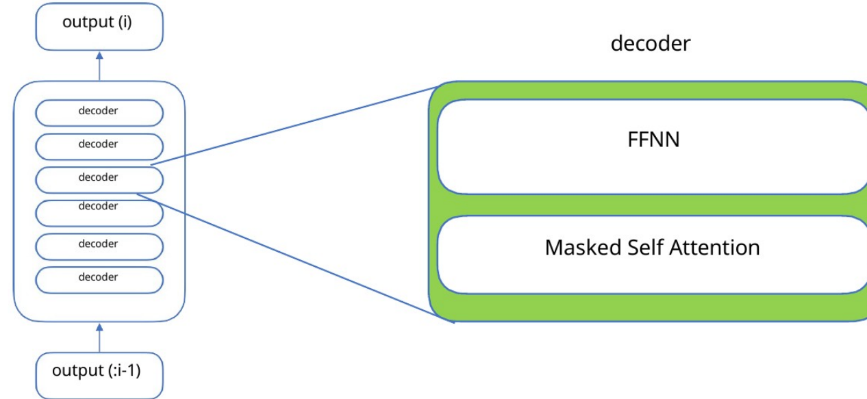
Architecture: Decoder only Transformer
