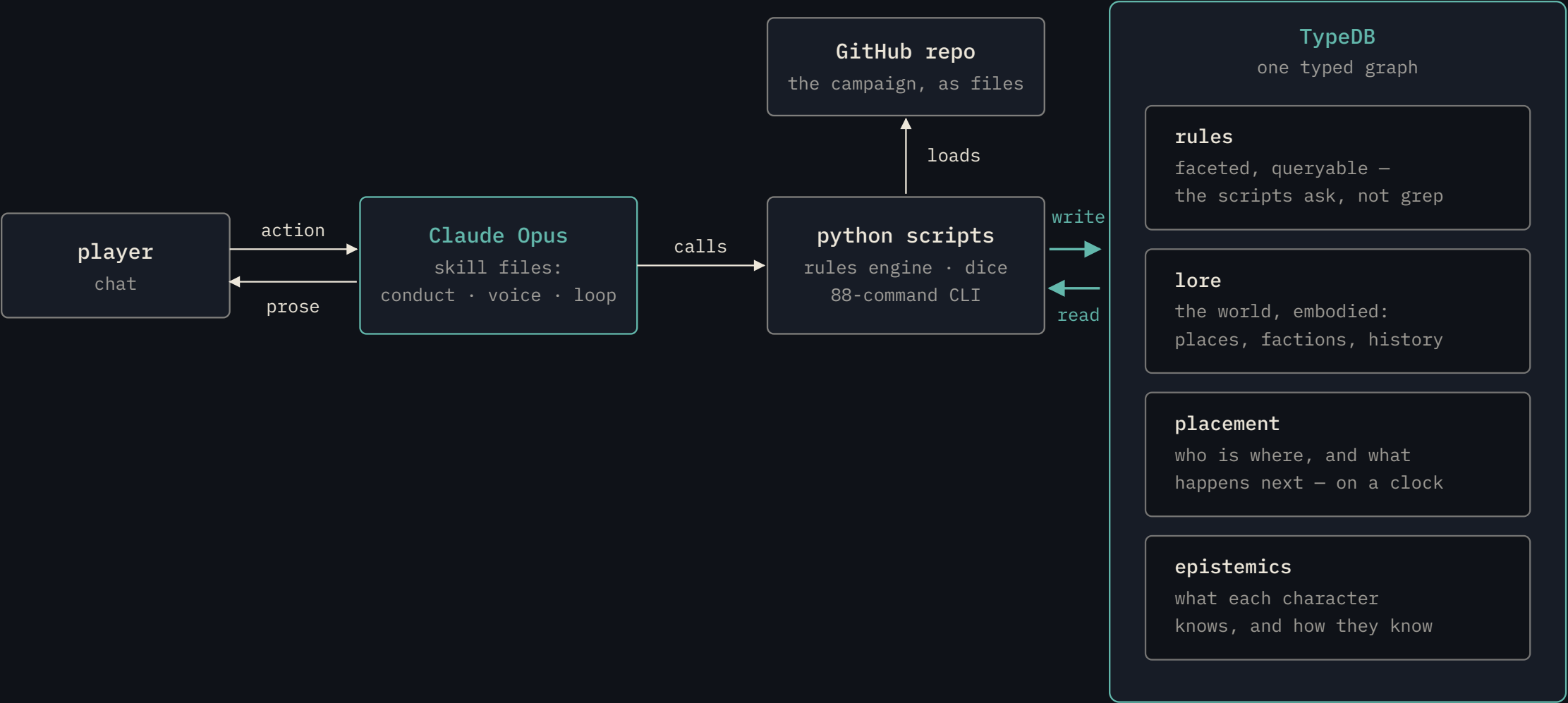
High-level data architecture of the game system, based only on agentic skills with a TypeDB structured memory store.
