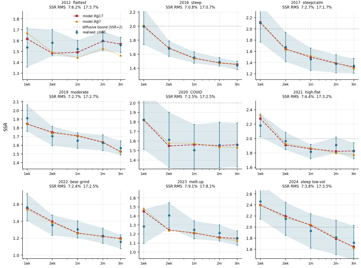
SPX realised SSR term structure ( \pm HAC) vs model — \theta@7 (stage 1) vs \theta@17 (stage 2)
