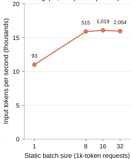
Throughput, W4 (labels: p50 ms)
