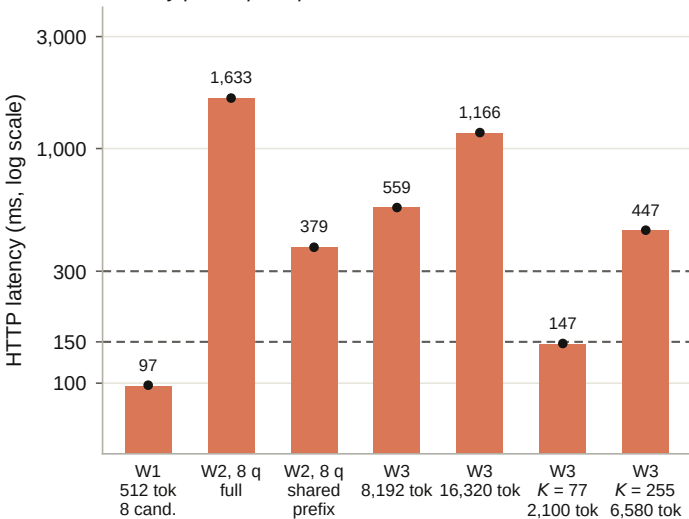
Latency per request profile
