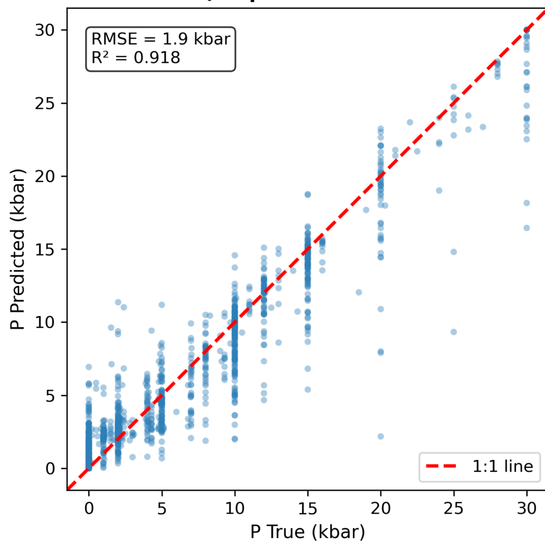
d) Liquid — Pressure
