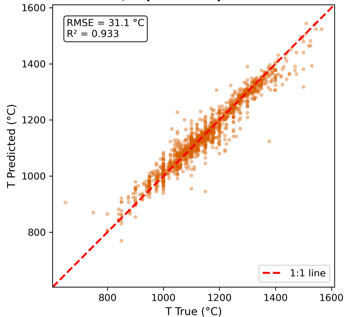
b) Liquid — Temperature
