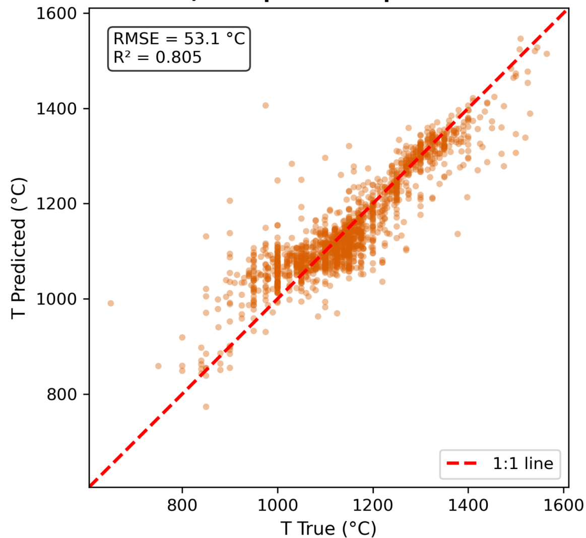
a) NoLiquid — Temperature
