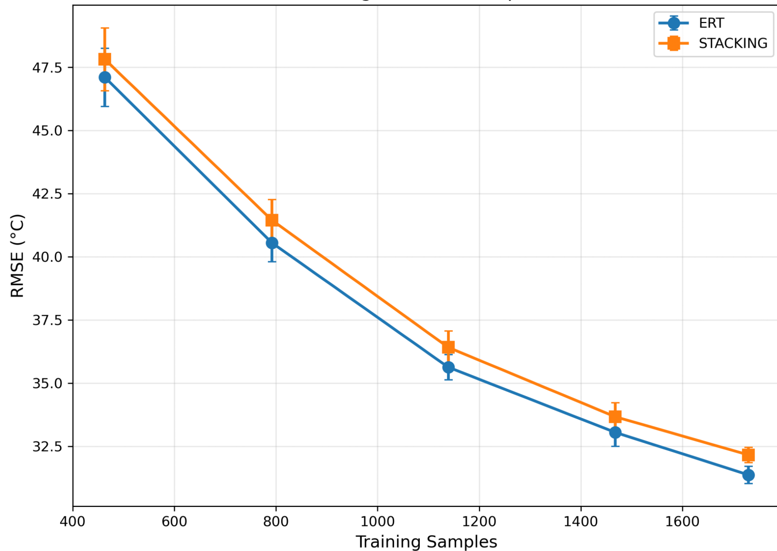
a) Learning Curve — Temperature
