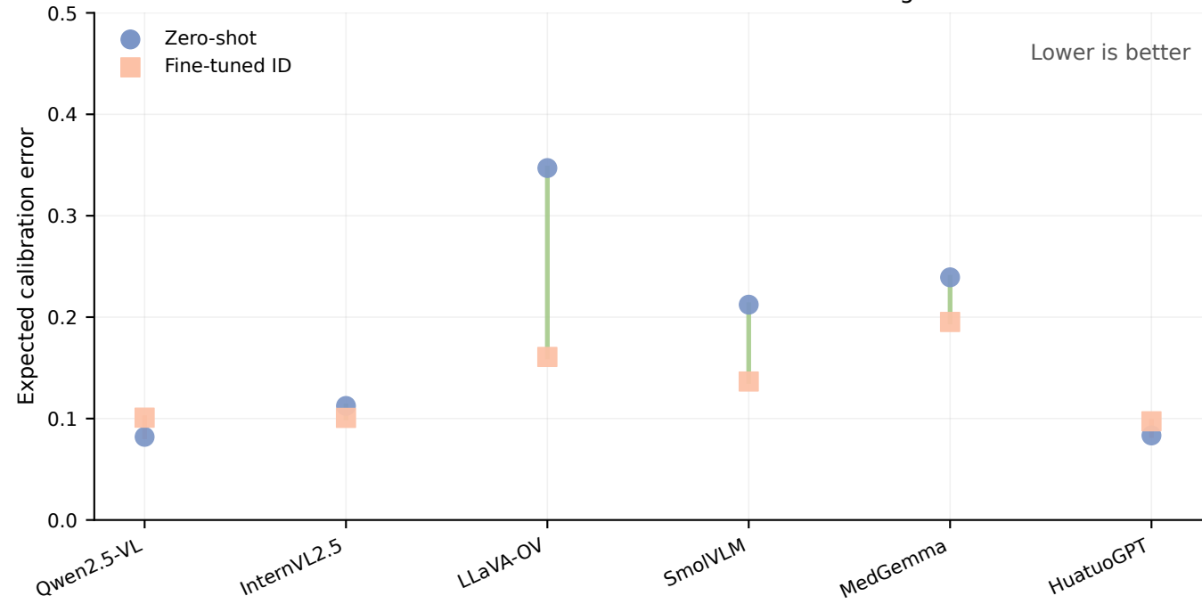
Calibration before and after LoRA fine-tuning
