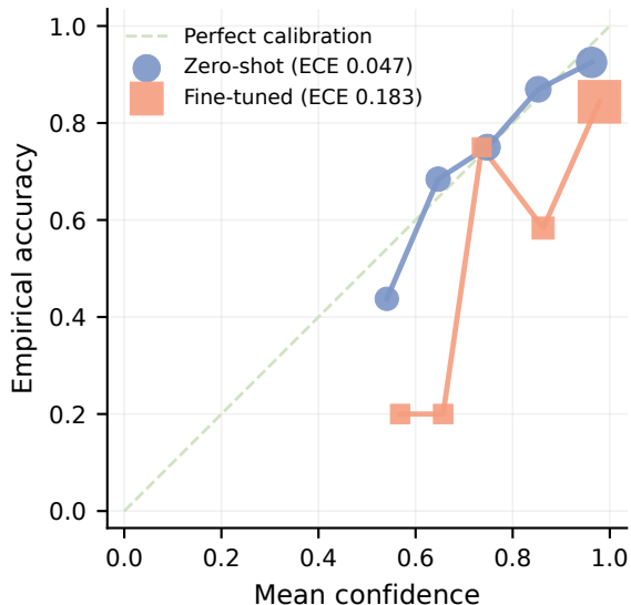
A. Fine-tuning can worsen calibration
