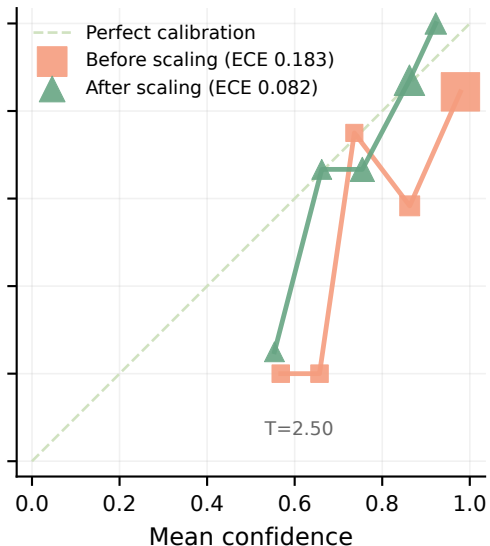
B. Temperature scaling pulls confidence back
