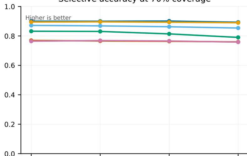
Selective accuracy at 70% coverage
