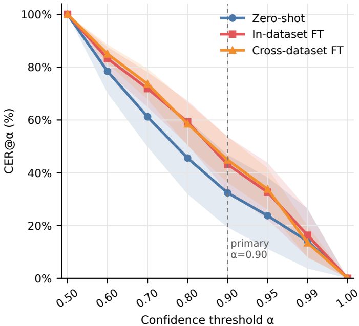
A. High-confidence error concentration
