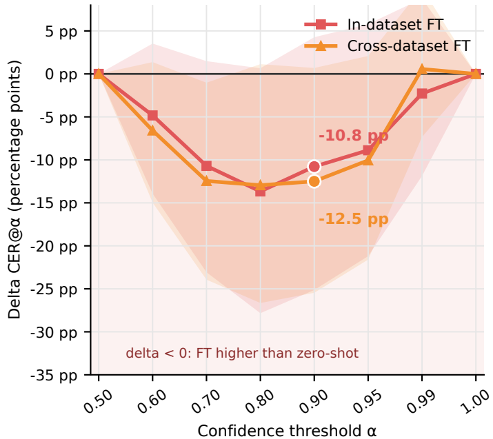
B. Delta relative to matched zero-shot
