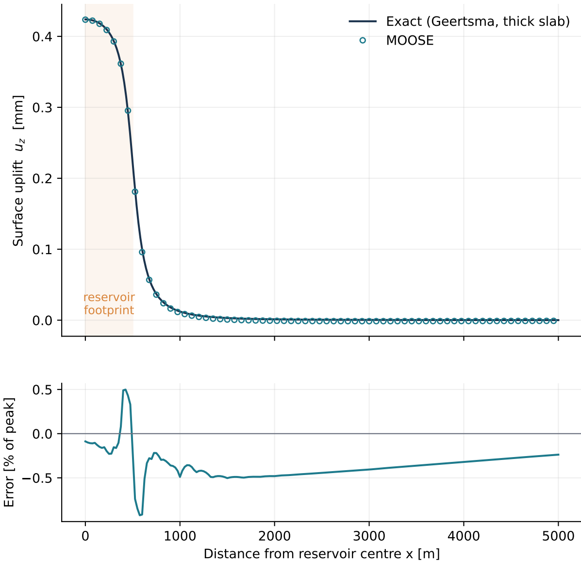
Geertsma benchmark: \Delta P = 1 MPa, reservoir 1 \times 1 km at 100-110 m depth
