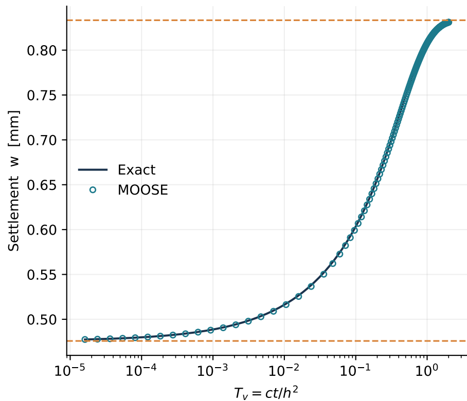
Surface settlement
