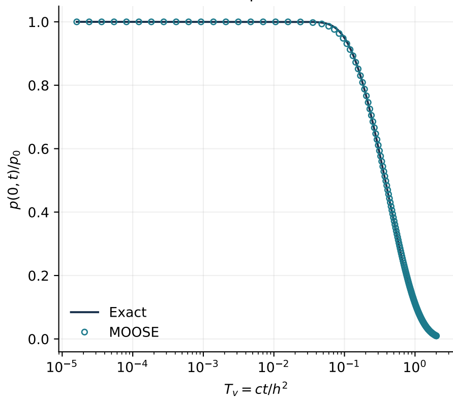
Pressure at impermeable base
