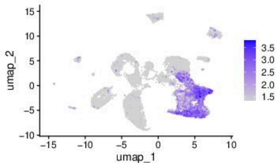
Mki67
