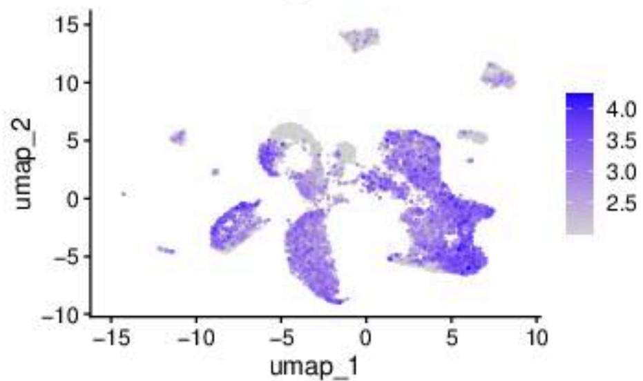
Rbfox1
