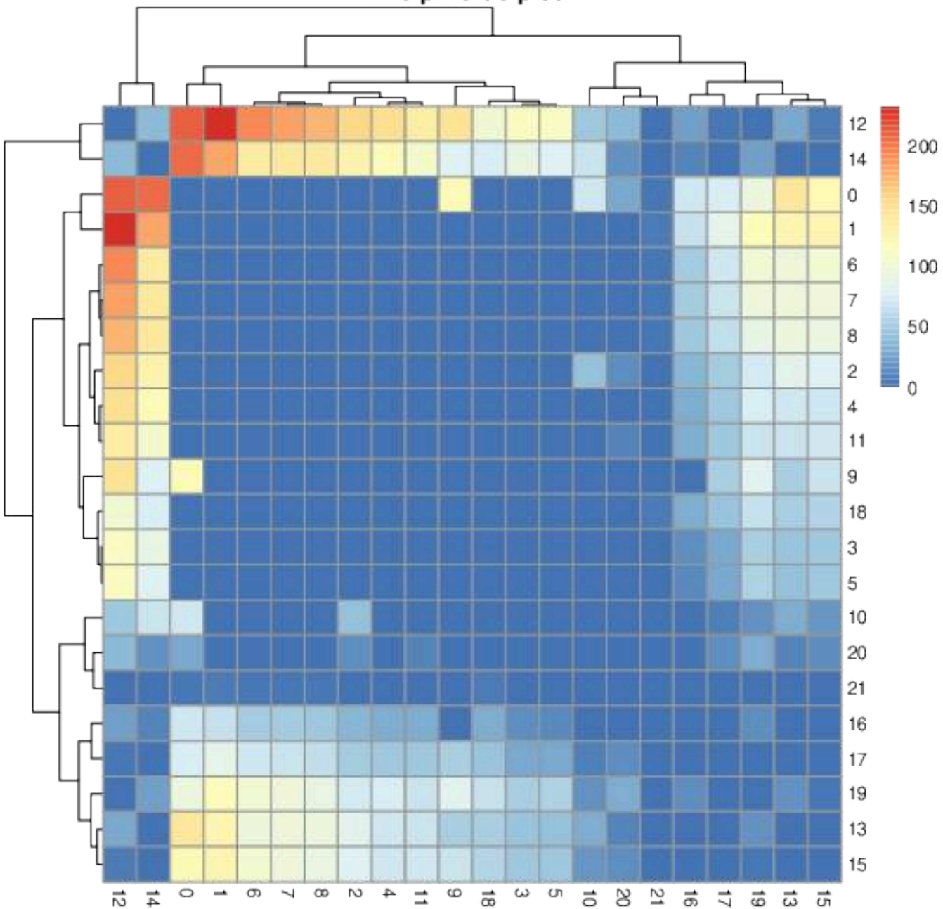
P0 p-value plot
