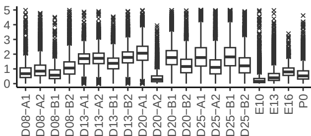
% mitochondria reads
