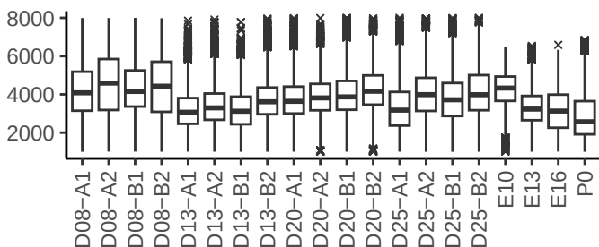
# genes detected
