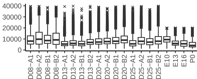
# transcripts detected
