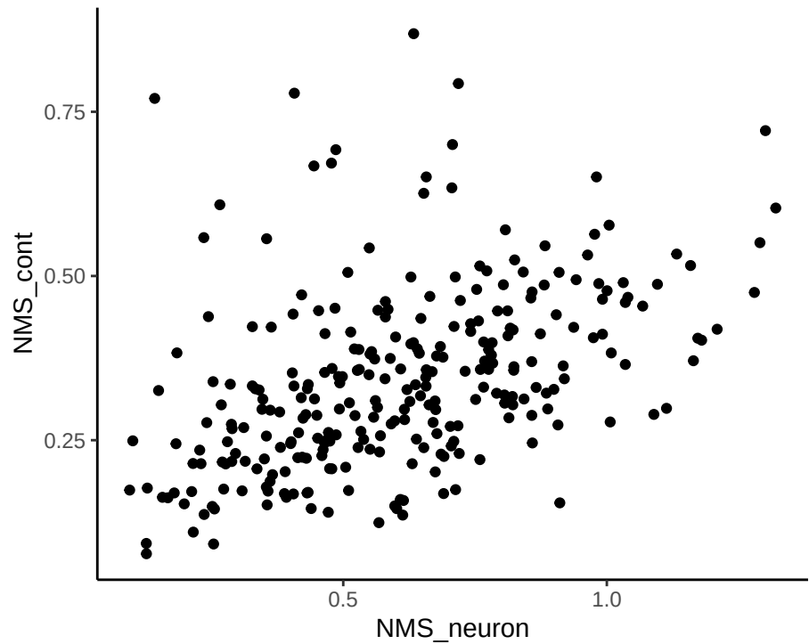
NMS plot
