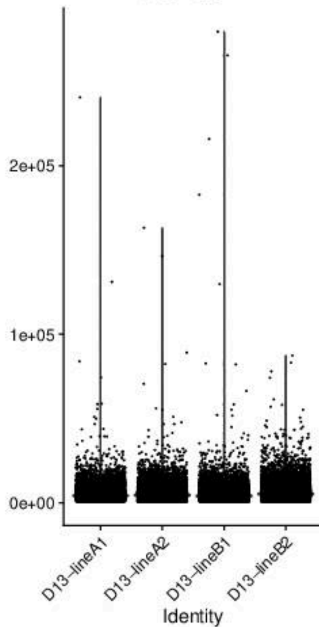
nCount_RNA
