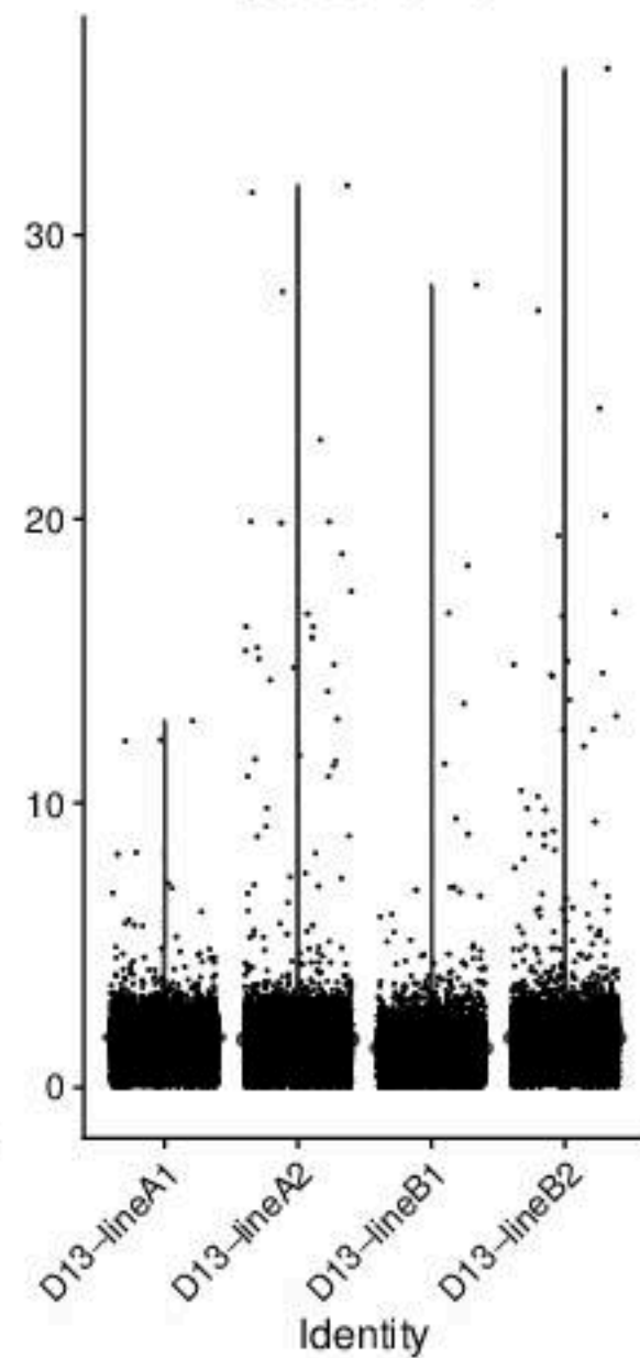
percent.mt
