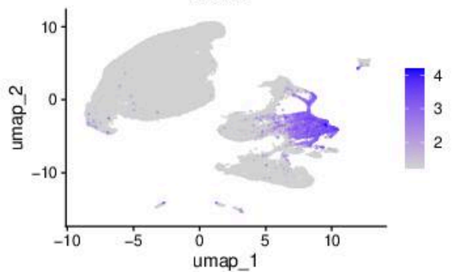
Mki67
