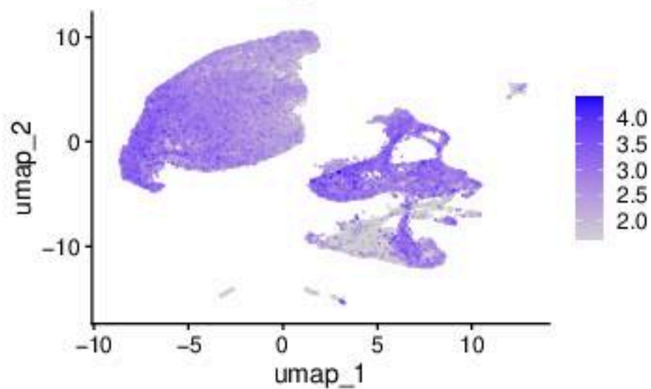
Rbfox1
