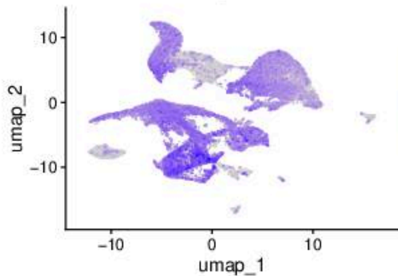
Rbfox1
