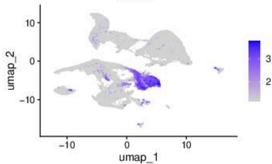
Mki67
