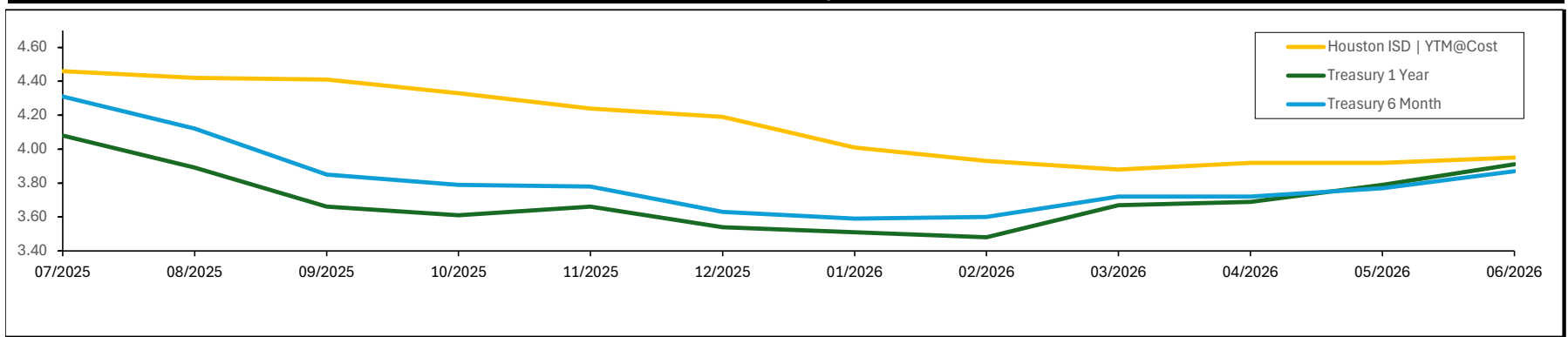
Performance Spread
