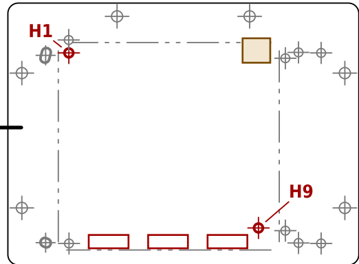
v3.2 (no shipped shuttle yet) board rev v3.2 offset X 19.40 Y 5.77 mm
