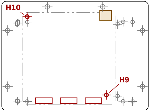
v3.3 (no shipped shuttle yet) board rev v3.3 offset X 19.40 Y 5.77 mm
