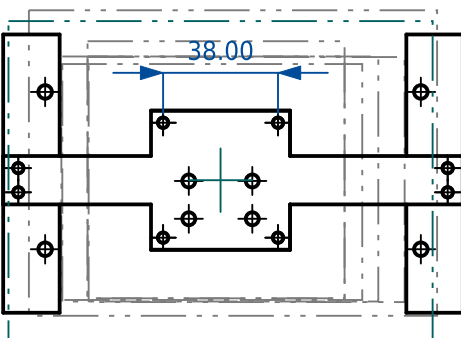
PLAN, 1:2.5, NOT IN PROJECTION
