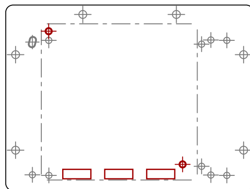
v3.3 (no shipped shuttle yet) board rev v3.3 offset X 19.400 Y 5.770
