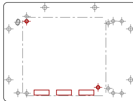
v3.2 (no shipped shuttle yet) board rev v3.2 offset X 19.400 Y 5.770
