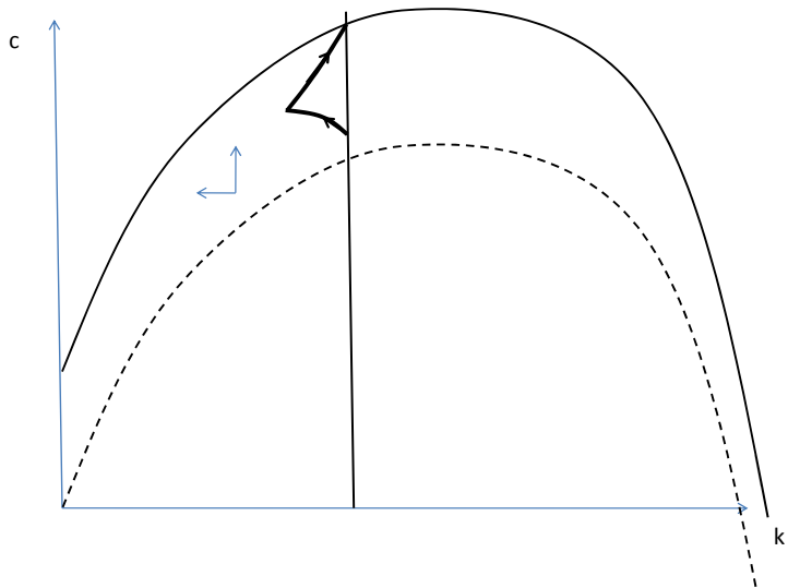
FIGURE 5 : Permanent anticipated manna from heaven
