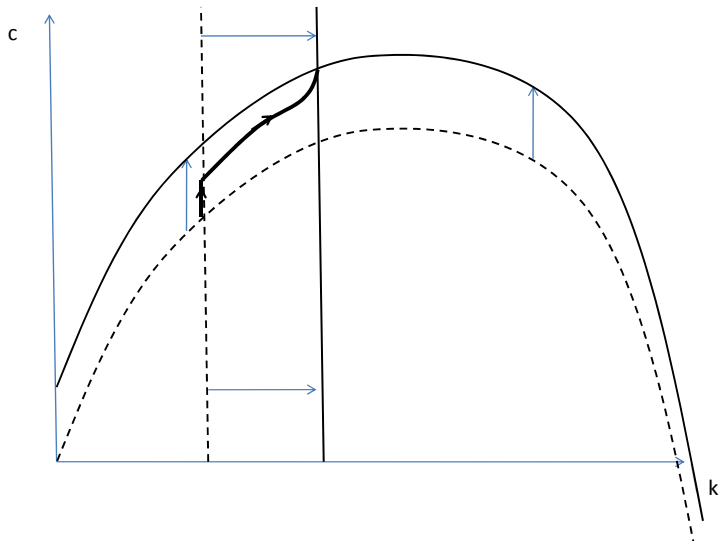
FIGURE 4 : Permanent multiplicative productivity shock
