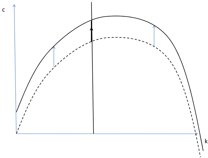
FIGURE 3 : Permanent manna from heaven
