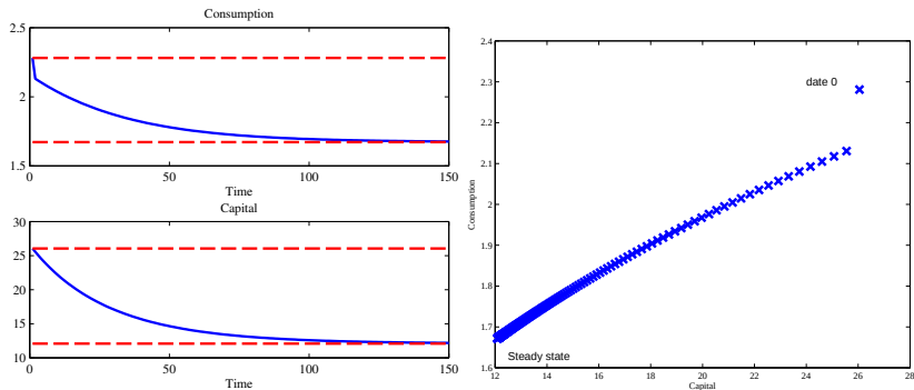
FIGURE 8 : Ramsey with depreciation shock - The case \sigma = 4 (low intertemporal substitution) (Note : On the right panel, each \times marker represents couple (k_t, c_t) for a given period t .)
