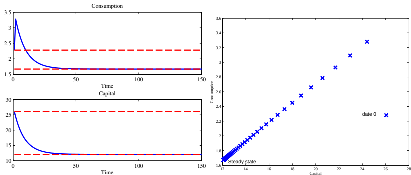
FIGURE 9 : Ramsey with depreciation shock - The case \sigma = .4 (high intertemporal substitution)(Note : On the right panel, each \times marker represents couple (k_t, c_t) for a given period t .)
