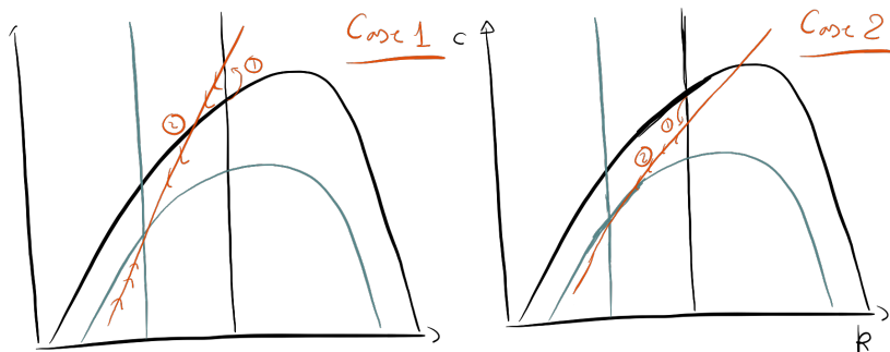
FIGURE 7 : Ramsey with depreciation shock - Possible paths
