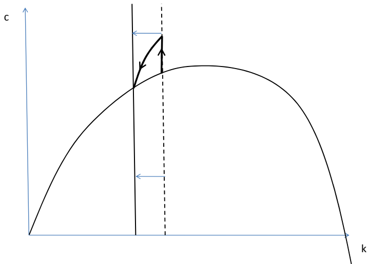
FIGURE 2 : Impact of a permanent rise in \rho
