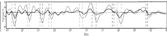
Fig. 3.11. Consumption (services).
