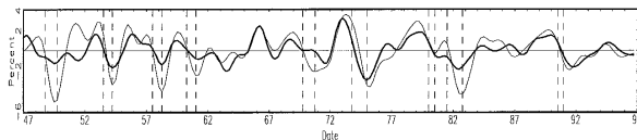
Fig. 3.10. Consumption (nondurables).
