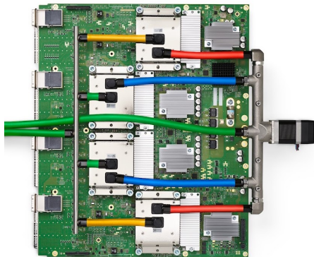
Google's Tensor Processing Unit (TPU)
