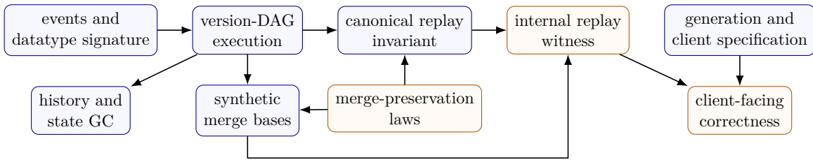
Figure 1: Semantic dependency order. Arrows point from prerequisite to consumer. The two GC layers are optional refinements, not premises of client-facing correctness.
