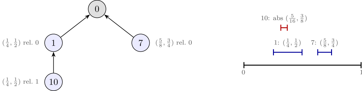
Figure 1: The state is a tree of deltas (left); absolute ranges are composed down the path (right): 10’s absolute range is \frac{1}{4} + \frac{1}{4} \cdot (\frac{1}{4}, \frac{1}{2}) = (\frac{5}{16}, \frac{3}{8}) . Display order: depth-first, children by descending range — newest first.
