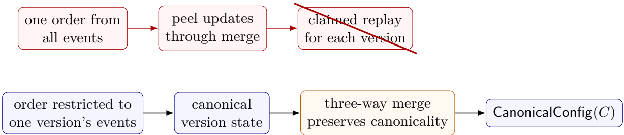
Figure 4: The refuted global-order argument and the repaired induction. The repaired path restricts ordering to one version's operations and asks each datatype to show that its three-way merge preserves the resulting state.
