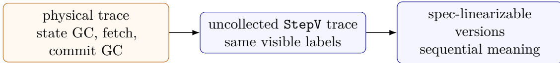
Figure 9: The two collectors remove different objects and compose by trace erasure. Commit GC removes versions; datatype GC removes metadata inside a retained state. The first arrow is GC.\text{CombinedSteps.refinesV} ; the second uses the VerifiedMRDT capstones.
