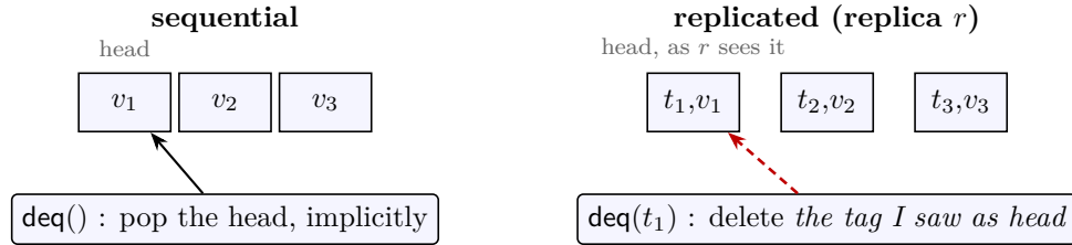
Figure 14: The observation gap, on the queue. The sequential dequeue is nullary; the replicated one names the tag its issuer read as the head of its own replica (dashed: the witness). Honesty is the faithfulness of the witness: qOK states that the fold at the issue point is literally (t_1, v_1) :: \text{rest} .
