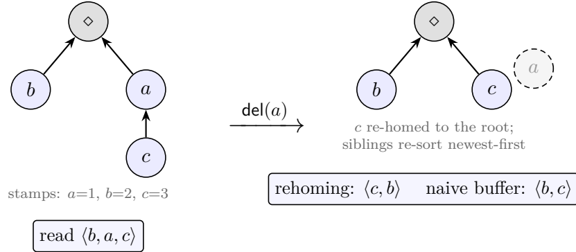
Figure 16: The four-op refutation. One replica, no merge. Deleting a swaps the surviving b and c in the rehoming RGA’s read; the naive buffer keeps their order. The embedded-chain RGA reads \langle b, c \rangle on the same trace: c ’s immutable coordinate still carries a ’s chain as pure geometry, so nothing moves.
