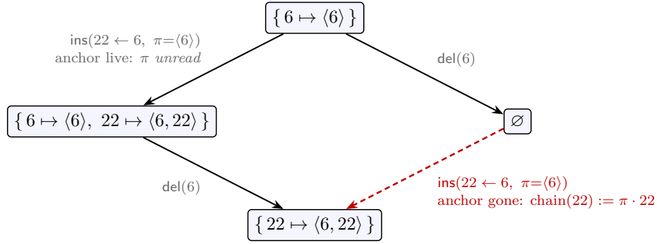
Figure 11: \text{rc} = \text{Either} discharged: \text{ins}(22 \leftarrow 6) and \text{del}(6) commute to equality . Down the left, the anchor is live and application never consults \pi (the reachable, honest order). Down the right, 6 is already gone: the state cannot supply the anchor's chain, so the carried \pi = \text{chain}(6) does, landing 22 on the same sort key. The right-hand state is unreachable under honesty; the verification condition quantifies over it anyway, and \pi exists exactly to make that corner total.
