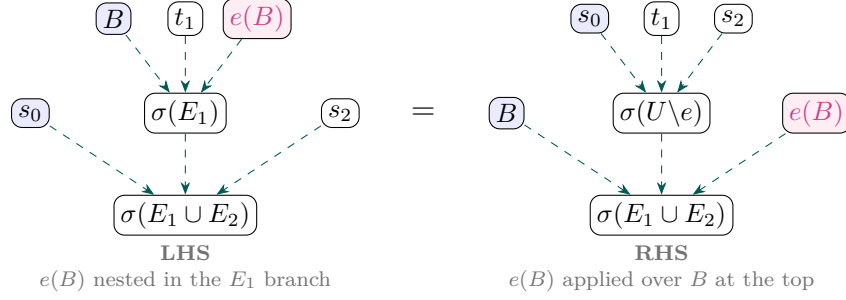
Figure 4: Flat VC 6 (VC6) read as an equation between two merge arrangements (dashed arrows feed each ternary mergel ; its shaded input is the LCA slot). The lo -maximal event e lies in one branch. LHS : e enters buried in the E_1 branch as its delta e(B) over the past it saw, B = \sigma(\downarrow e \setminus \{e\}) , with t_1 = \sigma(E_1 \setminus \{e\}) the rest of that branch and s_2 = \sigma(E_2) the far branch; the reconstructed branch \sigma(E_1) then merges under the LCA s_0 = \sigma(E_1 \cap E_2) . RHS : the same delta is pulled out and applied once at the enclosing merge, whose LCA slot is now B and whose middle input is the e -free merge \sigma(U \setminus e) = \text{mergel}(s_0, t_1, s_2) . The VC is exactly the claim that the two arrangements agree; both yield \sigma(E_1 \cup E_2) .
