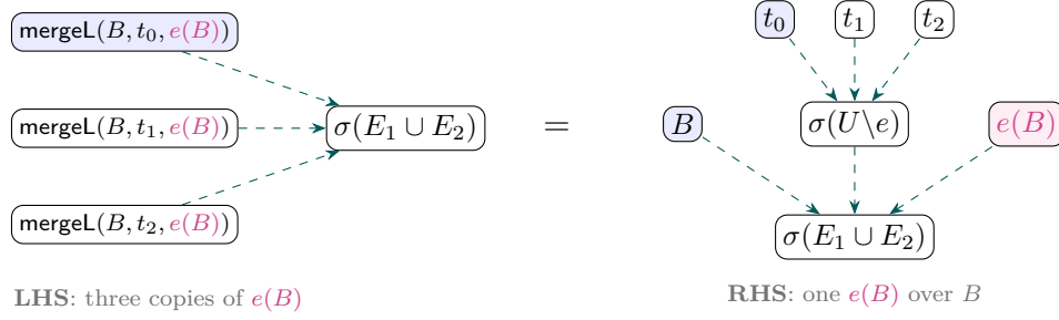
Figure 5: Flat VC 7 (VC7) read as an equation (dashed arrows feed each ternary mergeL ; its shaded input is the LCA slot). The \text{lo} -maximal event e lies in the LCA and both branches, so its delta e(B) over the shared past B = \sigma(\downarrow e \setminus \{e\}) sits in all three inputs ( mergeL ( B, t_i, e(B) ), with t_i the e -free rest). LHS : three copies of that delta, one per input. RHS : the triple count cancels and VC 7 factors them to a single e(B) over B , applied once at the enclosing merge over the e -free join \sigma(U \setminus e) = \text{mergeL}(t_0, t_1, t_2) , the ternary stand-in for idempotence. Both arrangements yield \sigma(E_1 \cup E_2) .
