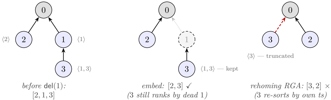
Figure 1: The one-line separation on the L1 delete-reorder litmus: insert 1 and 2 at the front, 3 after 1, delete 1. The rehoming RGA’s climb (red) re-parents 3 and re-sorts it by its own timestamp — the truncated key \langle 3 \rangle beats \langle 2 \rangle , and 3 jumps over 2. The embedded chain \langle 1, 3 \rangle keeps ranking 3 by its dead parent’s timestamp: [2, 3] , the delete-order-preserving read. Arrows point from a node to its anchor; dashed grey = dead.
