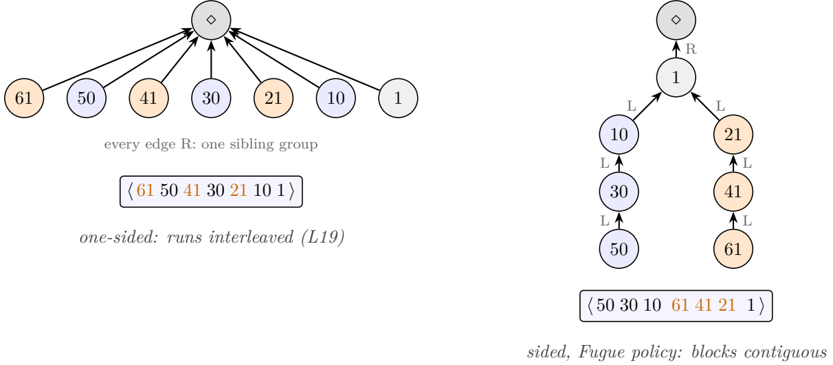
Figure 14: L19 under the two anchoring rules, the battery’s own trace. LCA document \langle 1 \rangle ; replica A (blue) types backward 10, 30, 50 before the head while replica B (orange) concurrently types backward 21, 41, 61. One-sided (left): every insert-before anchors at the same left neighbor \diamond , both runs land in one R-sibling group, and the timestamp-sorted fan interleaves them. Sided under the Fugue policy (right): insert-before anchors at the successor as an L-entry, each run is an L-chain hanging off 1, and the in-order read keeps the blocks contiguous: L-extensions precede the node (50, 30, 10 before their parents’ line ending at 1), and among the L-siblings 10, 21 of node 1 the older run displays first (the L band is mirrored). Both display strips are outputs of the sided model harness, embed_sided.py .
