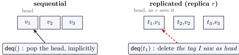
Figure 16: The observation gap, on the queue. The sequential dequeue is nullary; the replicated one names the tag its issuer read as the head of its own replica (dashed: the witness). Honesty is the faithfulness of the witness: qOK states that the fold at the issue point is literally (t_1, v_1) :: \text{rest} .
