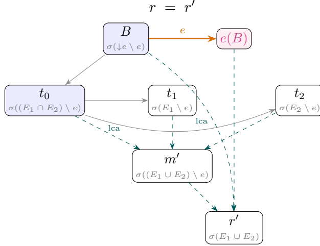
Figure 5: Flat VC 7 (VC7), conventions as in Figure 4. Here the lo-maximal event e lies in the LCA and both branches. Top (LHS): its delta e(B) enters all three inputs of the Join-Lemma merge, each m_i rebuilt at LCA B from the e -free t_i ; the three then merge at LCA m_0 . Bottom (RHS): the e -free world merges first at LCA t_0 into m' , and a single copy of the delta applies on top, at LCA B : the triple count cancels, the ternary stand-in for idempotence. The VC is the equation r = r' : both realize \sigma(E_1 \cup E_2) .
