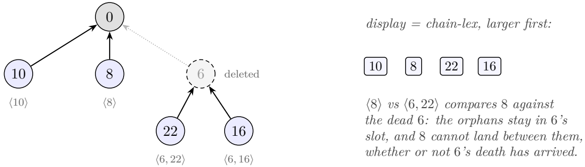
Figure 8: The credential countermodel as a birth tree. 6 and 10 race at the front; 22, 16 are typed under 6; 6 dies; 8 arrives at the front concurrently. Survivors sort by whole birth chains, so the read is [10, 8, 22, 16] at every replica and merge order. Every timestamp-oblivious variant flips this shape (§29).
