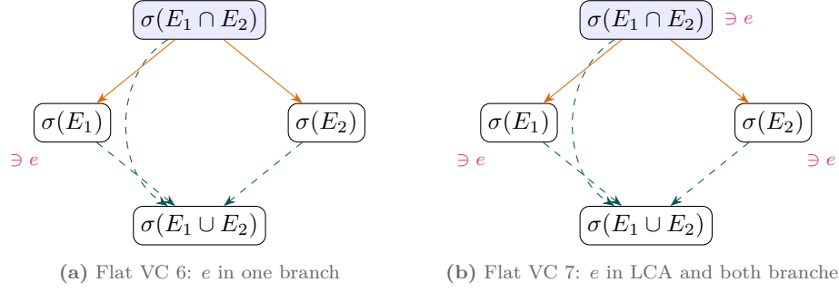
Figure 4: The peel of the lo-maximal event e from the Join Lemma’s three-way merge: the LCA \sigma(E_1 \cap E_2) (shaded) and the branches \sigma(E_1) , \sigma(E_2) merge to \sigma(E_1 \cup E_2) (solid arrows apply a branch’s events, dashed arrows feed the merge). (a) Flat VC 6 peels e (magenta) when it lies in one branch: its delta slides out over the merge, applied over its own past B = \sigma(\downarrow e \setminus \{e\}) . (b) Flat VC 7 peels e when it lies in the LCA and both branches: its three copies factor out once.
