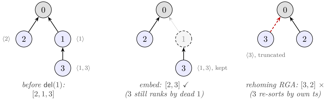
Figure 7: The one-line separation on the L1 delete-reorder litmus: insert 1 and 2 at the front, 3 after 1, delete 1. The rehoming RGA’s climb (red) re-parents 3 and re-sorts it by its own timestamp: the truncated key \langle 3 \rangle beats \langle 2 \rangle , and 3 jumps over 2. The embedded chain \langle 1, 3 \rangle keeps ranking 3 by its dead parent’s timestamp: [2, 3] , the delete-order-preserving read. Arrows point from a node to its anchor; dashed grey = dead.
