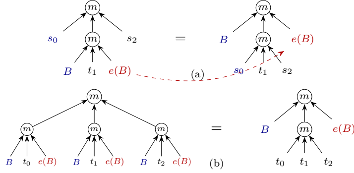
Figure 4: The two redistribute laws as peels of the lo-maximal event e from a ternary merge. Each node m is a mergeL (leftmost input the LCA slot, blue); red is e 's delta e(B) over its past B = \sigma(\downarrow e \setminus \{e\}) . (a) Flat VC 6: e in one branch slides out over the enclosing merge, leaving it e -free (over E_1 \cup E_2 \setminus \{e\} ). (b) Flat VC 7: e in all three inputs factors out once.
