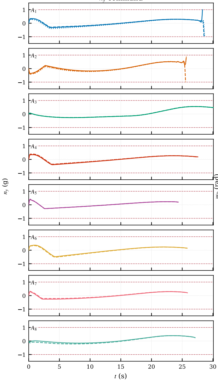
n_y command
