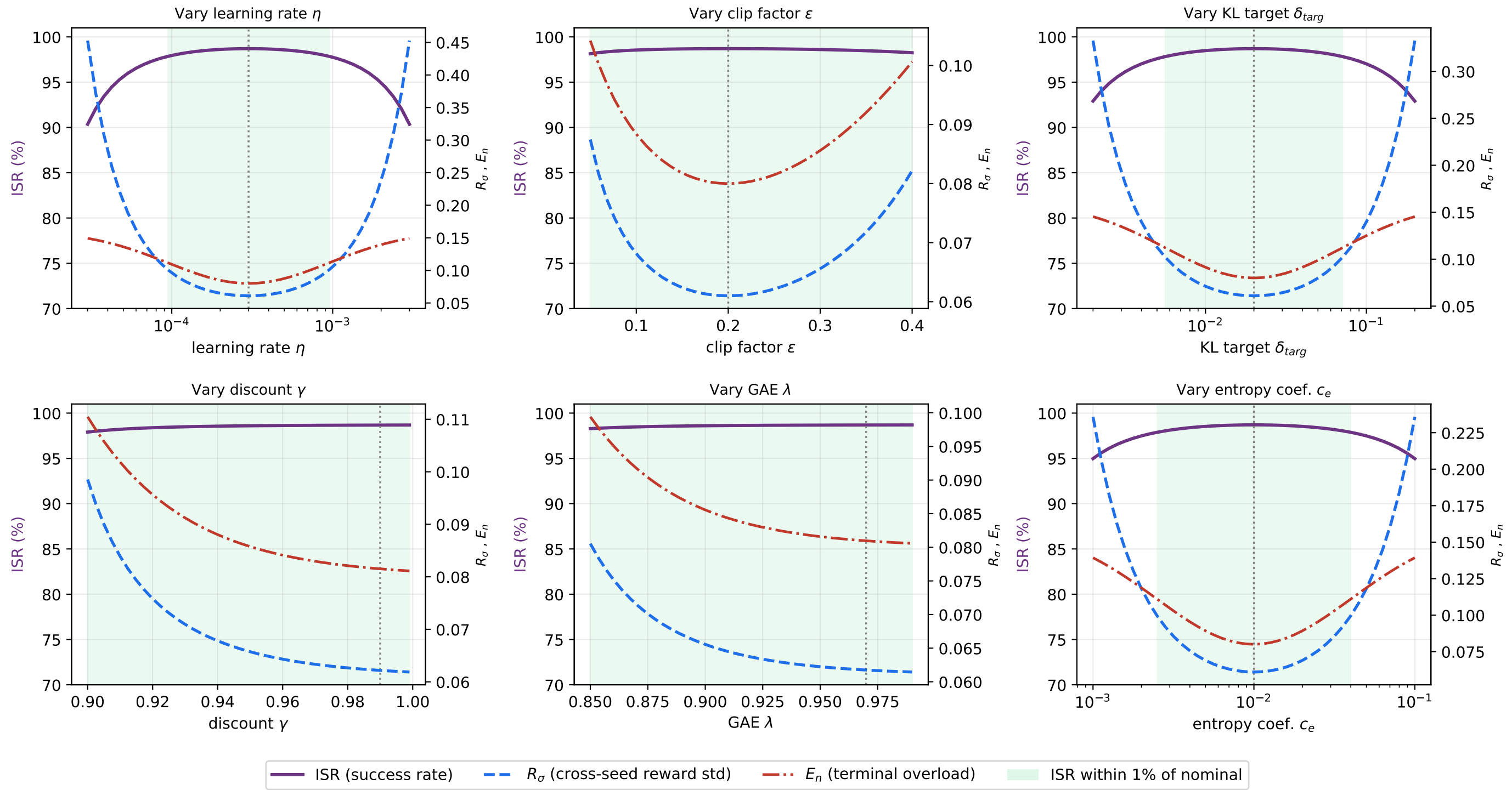
Sensitivity of ART-MAPPO training to its hyperparameters (anchored at the reported Case-1 operating point)
