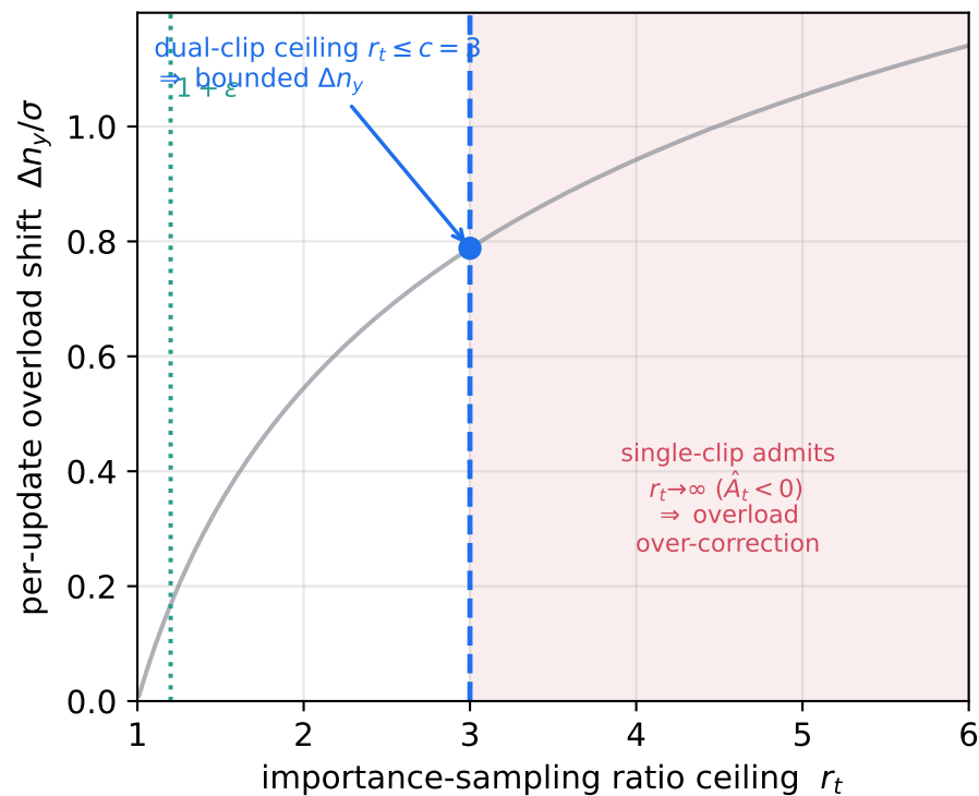
(b) dual-clip \Rightarrow load-factor guard
