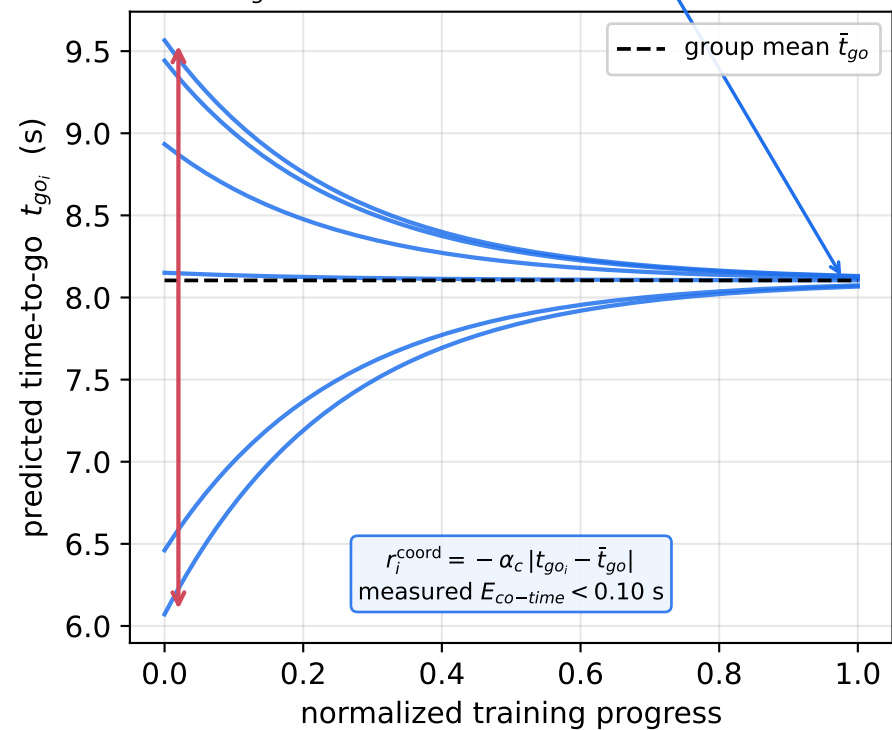
(a) t_{go} -consensus reward \Rightarrow salvo timing
