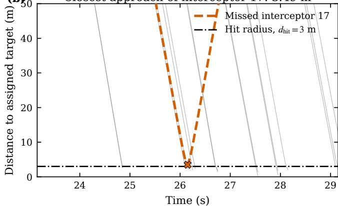
Closest approach of interceptor 17: 3.49 m
