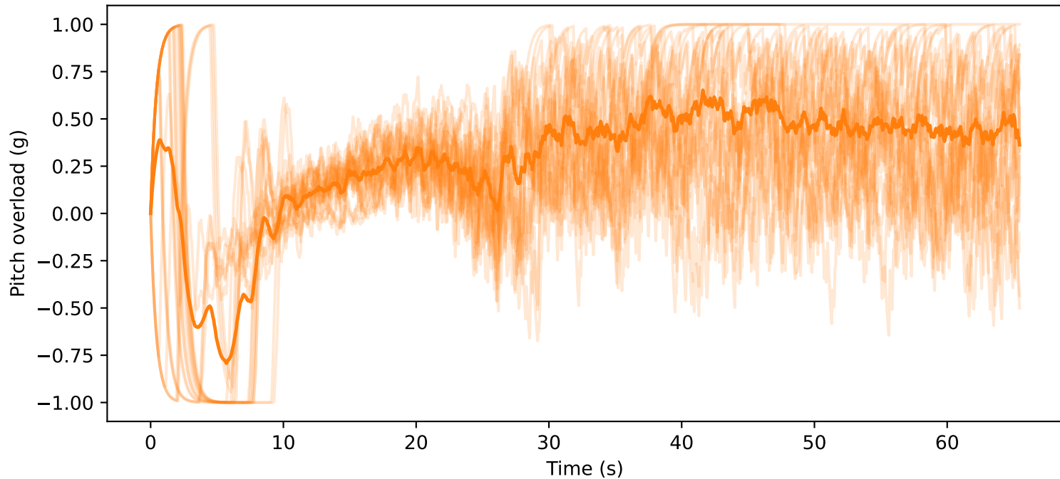
Case case2 Pitch Overload Command
