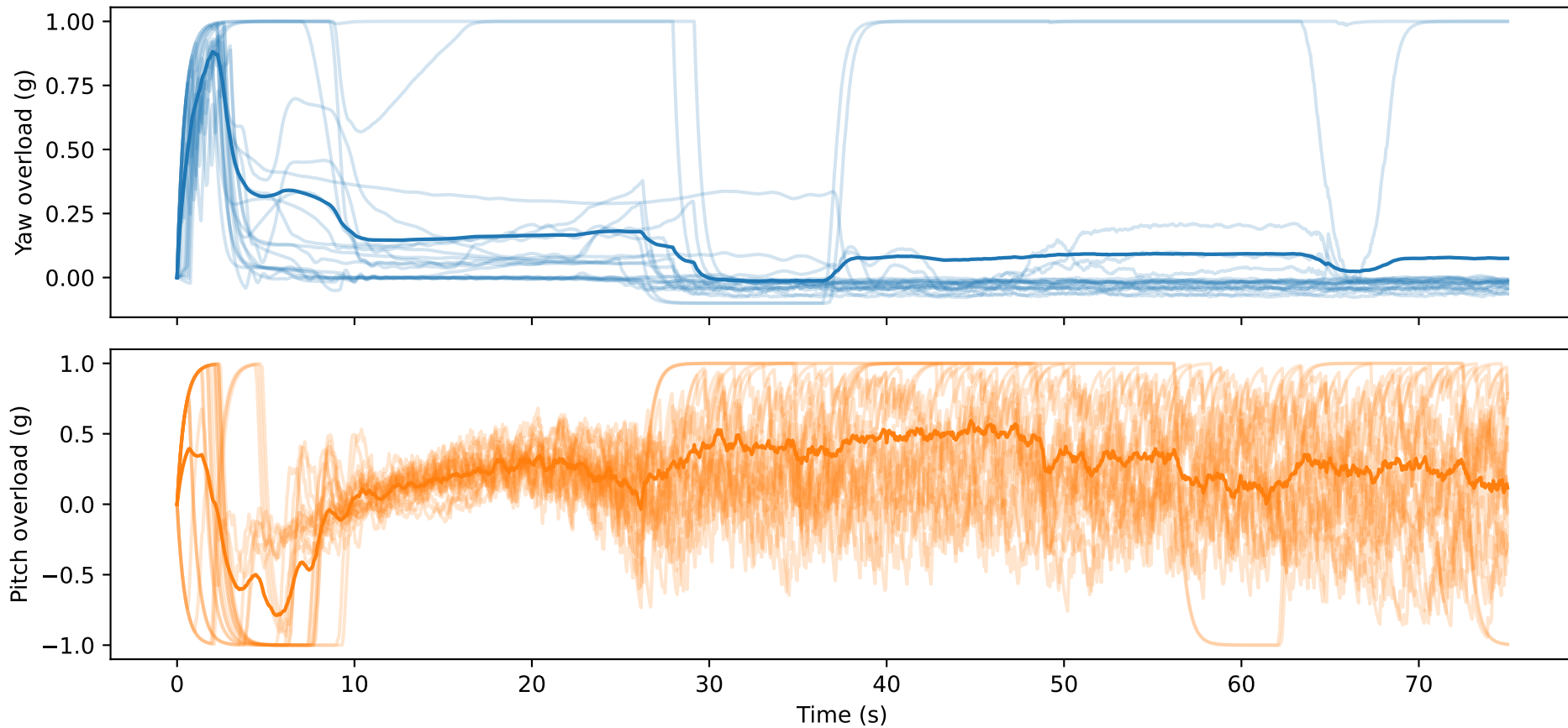
Case case2 Defender Commands
