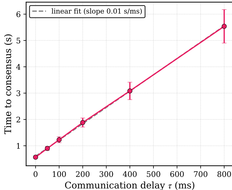
(b) Consensus time grows linearly with delay
