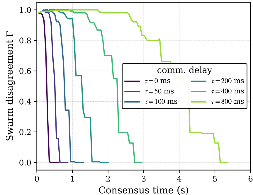
(a) Consensus under communication delay
