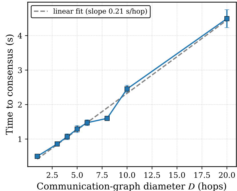
(c) Consensus time scales with graph diameter
