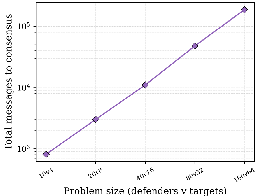
(b) Communication volume vs scale
