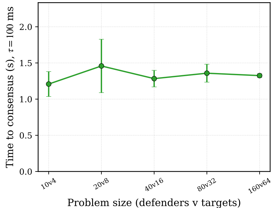
(a) Time-to-consensus vs scale
