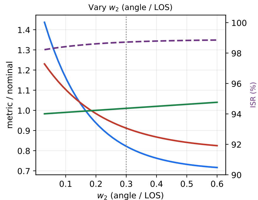
Reward-weight sensitivity of the four evaluation metrics (anchored at the reported Case-1 operating point)
