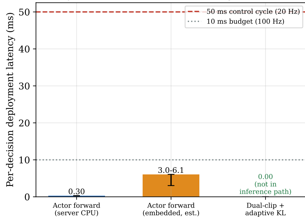
(a) Deployment cost vs. real-time budget (hidden=256)
